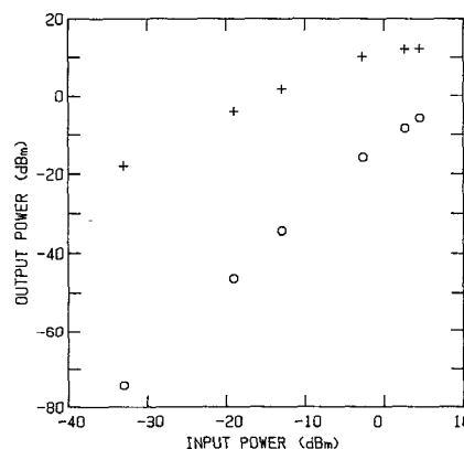
Figure 5 Gain Compression Characteristics of Common Source Amplifier with 15 dB small signal gain. Shown are the output powers contained in the fundamental frequency (10 GHz - +) and in the second harmonic (20 GHz - O).
